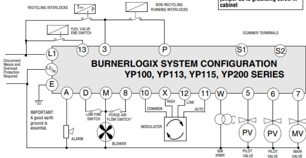
Note: When Flame Rod is used jumper S2 to grounding screw in cabinet
