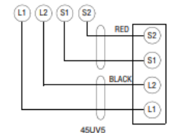
TYPICAL WIRING ARRANGEMENT FOR PILOT IGNITER (Applies to YP100 and YP 200 only)
