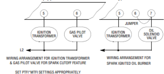
TYPICAL WIRING ARRANGEMENT FOR PILOT IGNITER (Applies to YP100 and YP 200 only)
