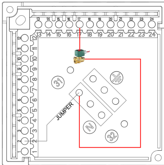
INTERRUPTED PILOT
